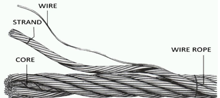
Wire Rope Technology
